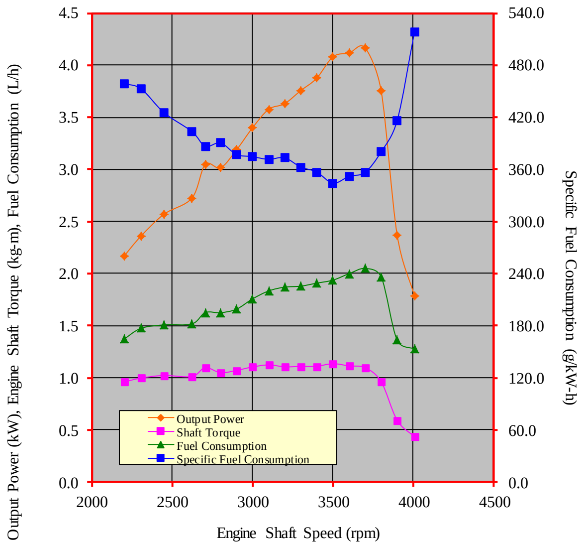
Figure 3. Performance characteristic curves of the PLATINUM KNM 65R gasoline engine
