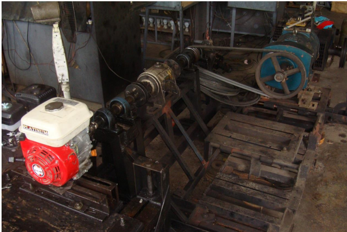
Figure 2. Test set-up of the PLATINUM KNM 65R Gasoline Engine
