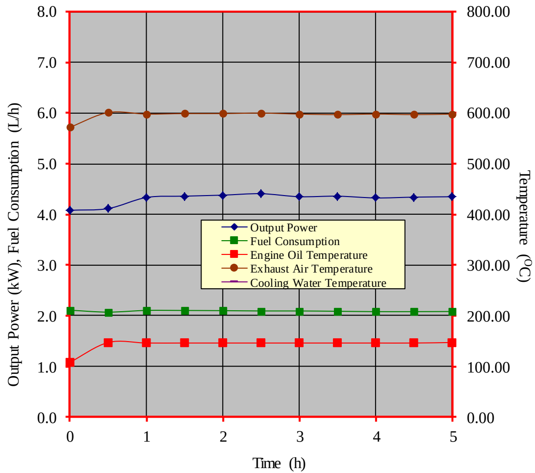
Figure 4. Performance characteristic curves during the continuous running test of PLATINUM KNM 65R gasoline engine
